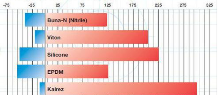
O-Ring Temperature Aptitude Graph (°C)
